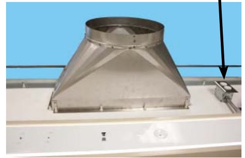
Integral stainless steel 12" round duct transition
