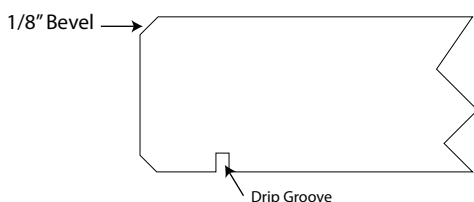
Standard Beveled Edge Finish Section view of work surface
