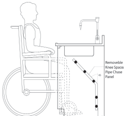
Section View
