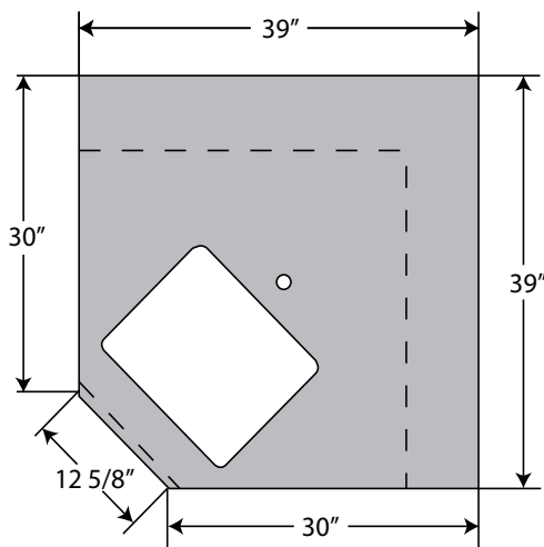
Plan View
